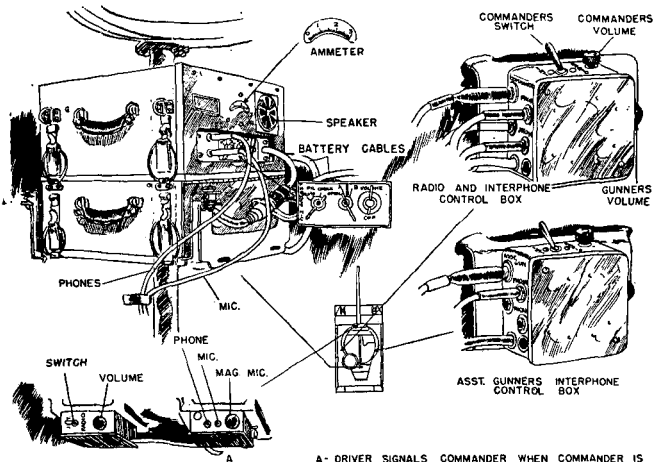
A - DRIVER SIGNALS COMMANDER WHEN COMMANDER IS OPERATING RADIO. DRIVER CAN SIGNAL HIM BY THROWING SWITCH TO INT. AND PRESSING MICROPHONE SWITCH. THIS PUTS TONE IN COMMANDERS HEADSET.
