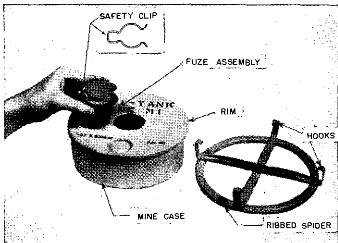
FIGURE 19.—Antitank mine.
