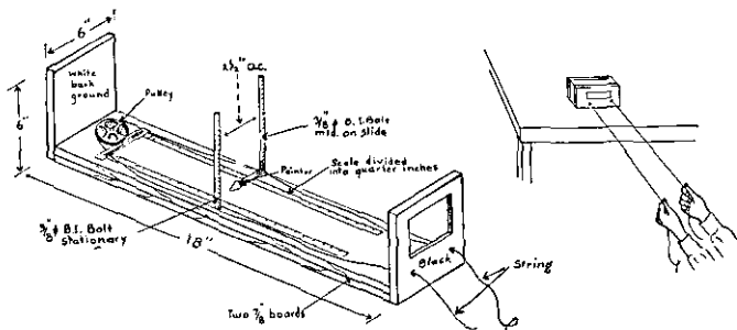
FIGURE 34.—Equipment for depth perception test.
