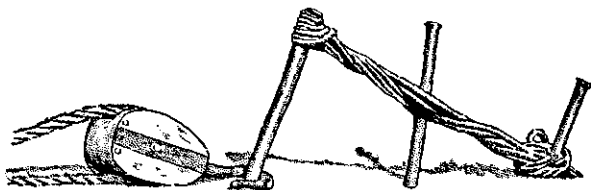
FIGURE 30.—Anchored stake.
