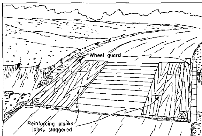
④ Additional planking and wheel guards. FIGURE 22.—Reinforcing bridges—Continued.
