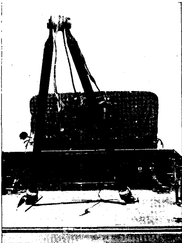
FIGURE 24.—Wrecking crane.
