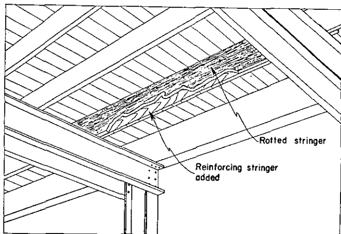
③ Added stringer.
