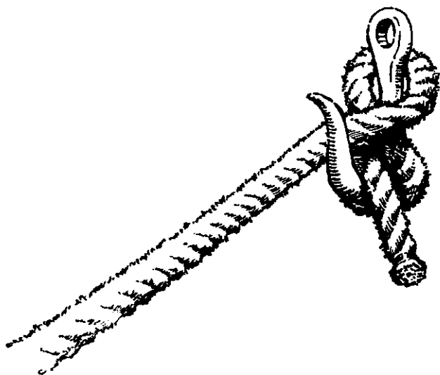
③ Double Blackwall knot.
