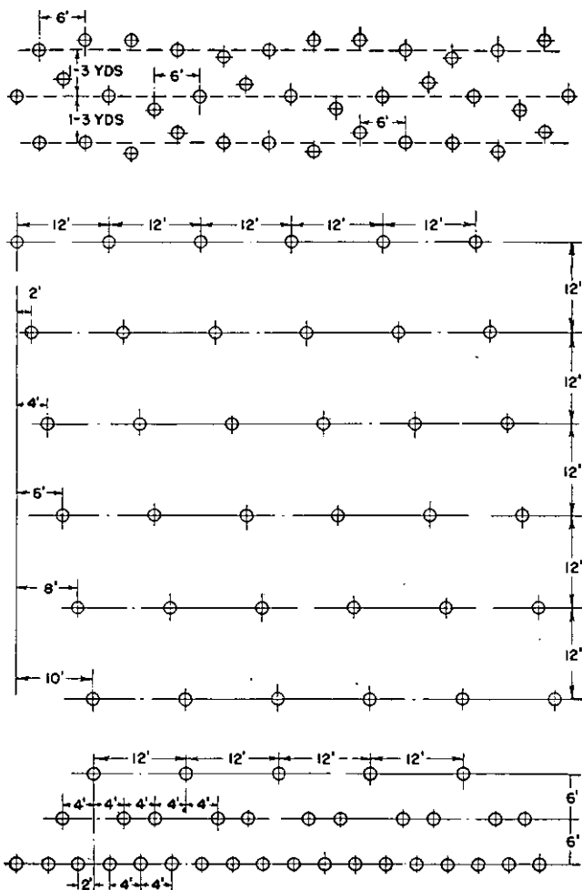
FIGURE 20.—Methods of arranging band of antitank mines.
