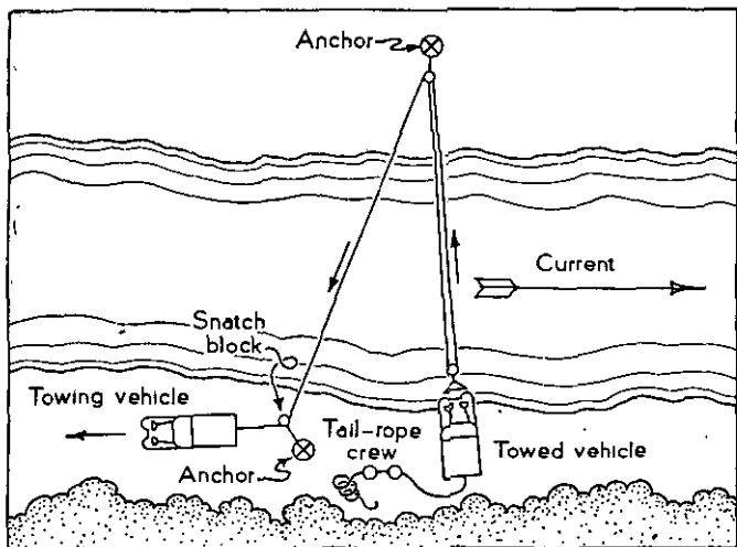
FIGURE 31.—Tackle for deep stream crossing.
