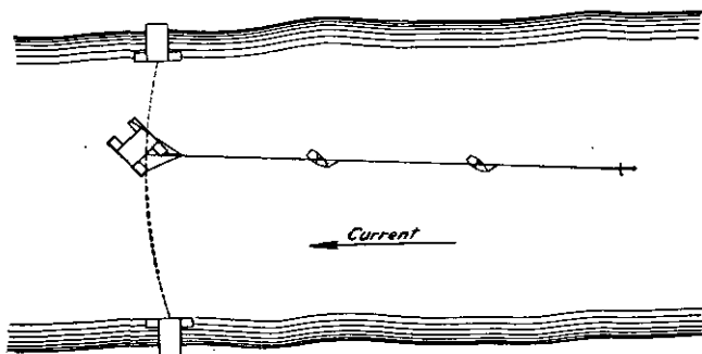
② Flying ferry.
