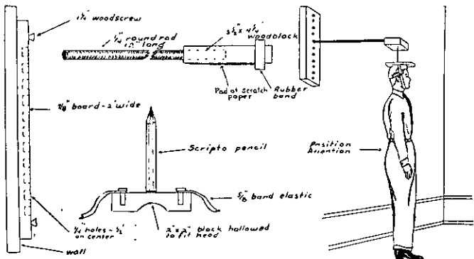
FIGURE 36.—Equipment for stability test.
