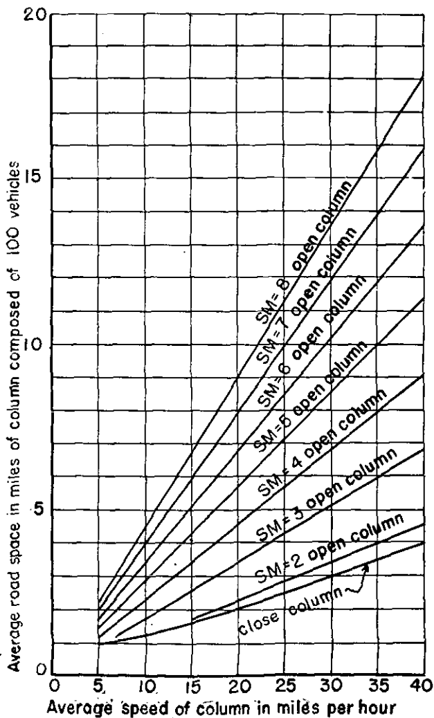
FIGURE 15.—Average road space of open and close motor columns at various speeds.
