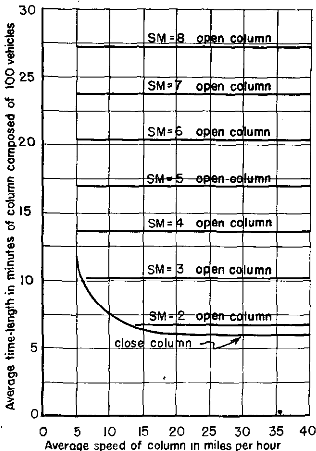
FIGURE 14.—Average time length of open and close motor columns at various speeds.
