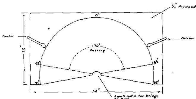
FIGURE 33.—Equipment for field of vision test.
