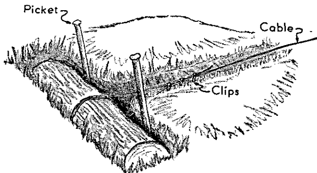
FIGURE 29.—Deadman installation.
