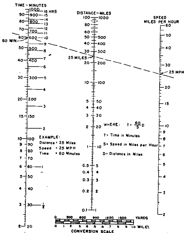
FIGURE 16.—Time, distance, and speed nomograph.
