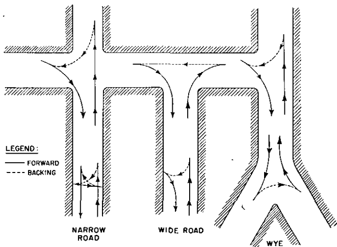
FIGURE 8.—Proper method of executing Y-turn when interfering traffic is blocked off.
