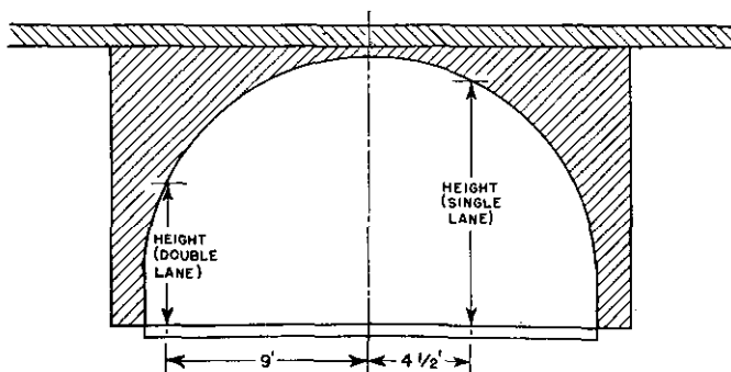
FIGURE 9.—Standard method of measuring vertical clearances under arches.
