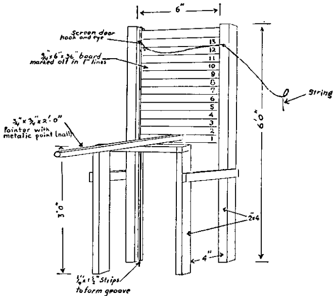
FIGURE 35.—Equipment for reaction test.
