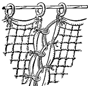
(2). — Quick-release device—ring and loop.
